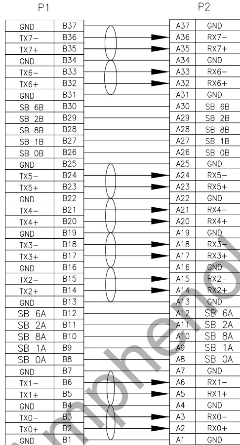
WIRE DIAGRAM
